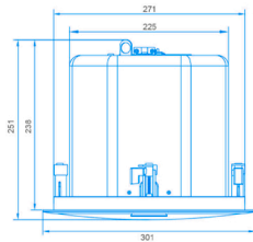
C8 Hole Size 271mm
