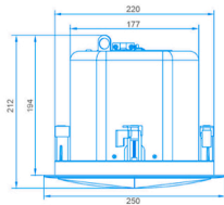
C6 Hole Size 220mm
