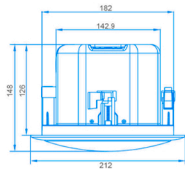
C4 Hole Size 182mm
